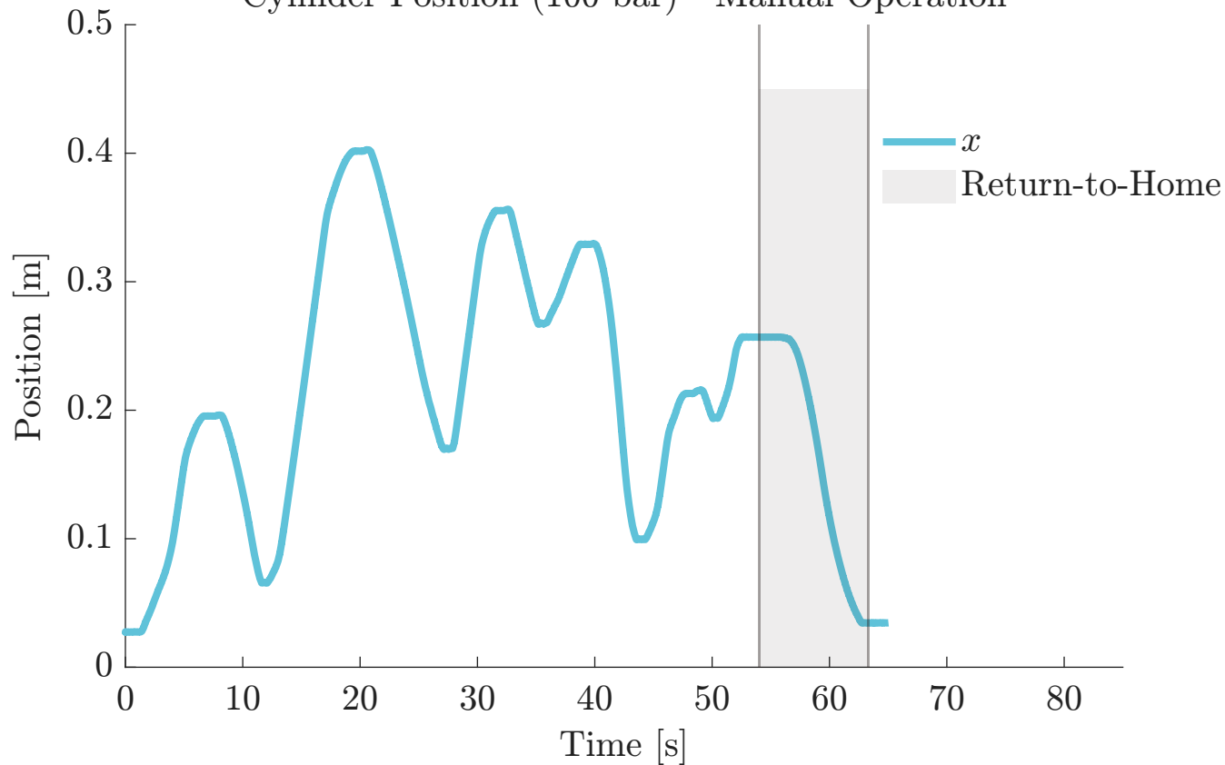
Cylinder Position (100 bar) - Manual Operation
