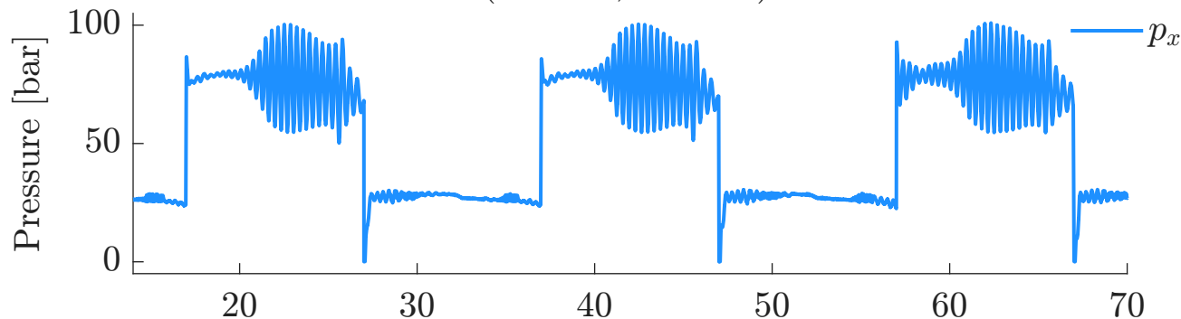
Pressure Feedback (120 bar, 0.05 Hz) - Pressure Gradient
