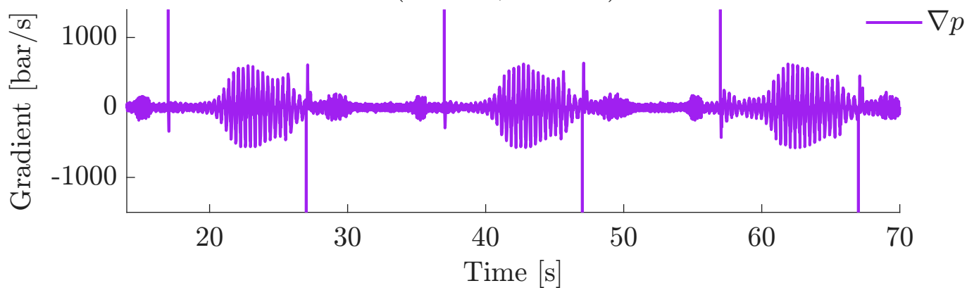
Pressure Feedback (120 bar, 0.05 Hz) - Pressure Gradient
