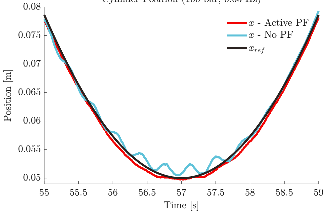
Cylinder Position (100 bar, 0.05 Hz)
