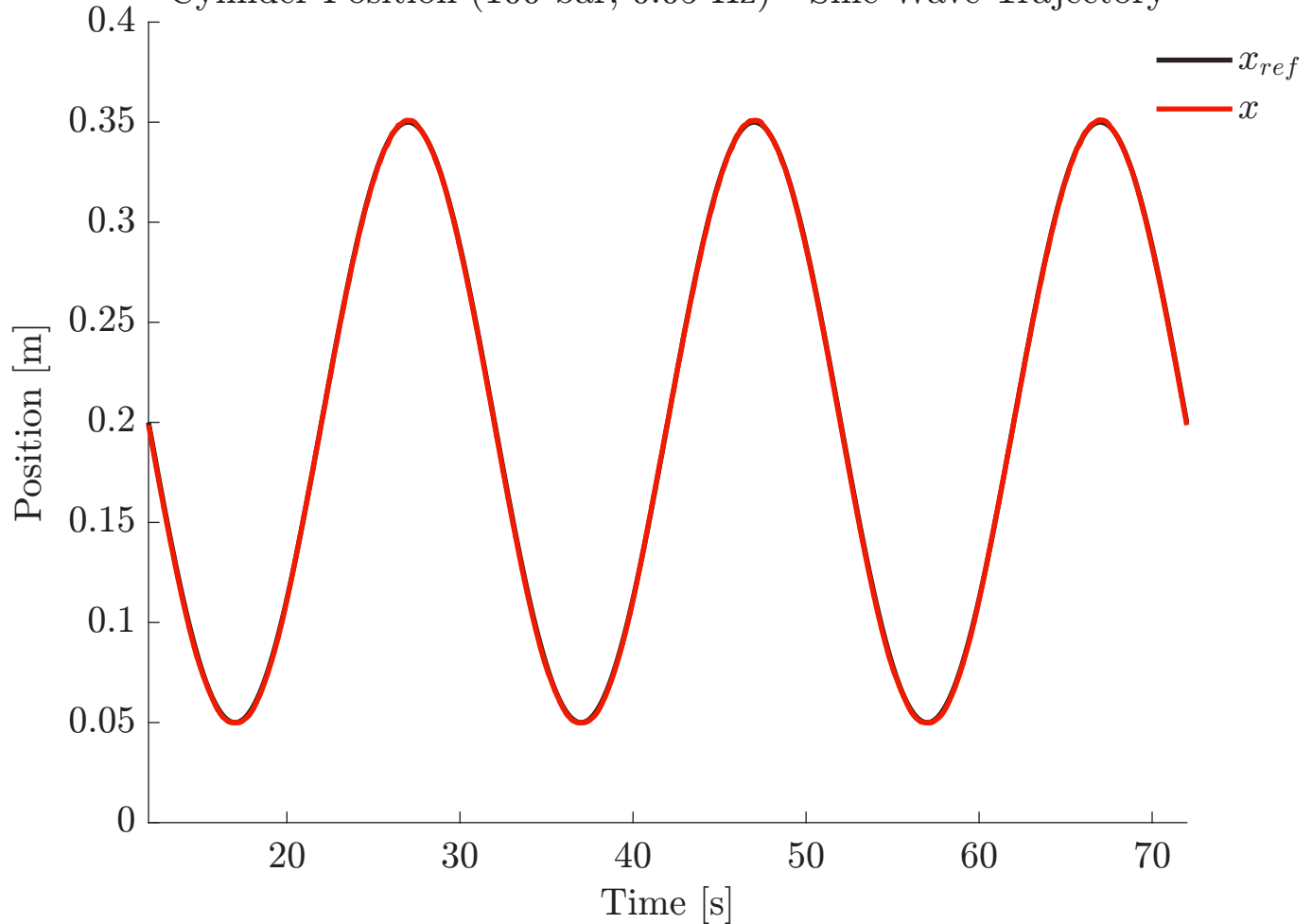
Cylinder Position (100 bar, 0.05 Hz) - Sine Wave Trajectory
