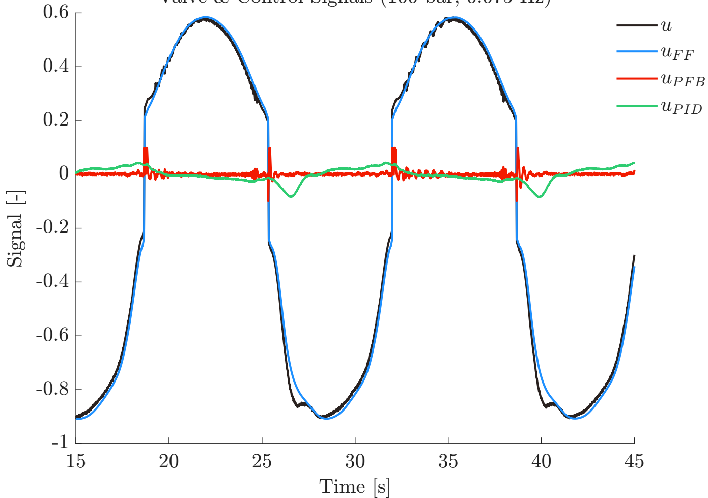
Valve & Control Signals (100 bar, 0.075 Hz)
