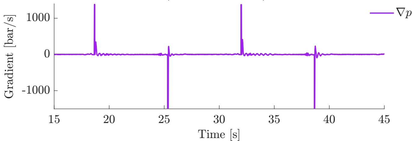
Pressure Feedback (100 bar, 0.075 Hz) - Pressure Gradient
