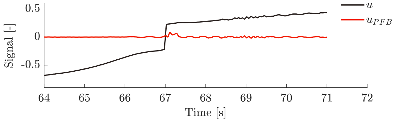
Pressure Feedback (100 bar, 0.05 Hz) - Valve Signals
