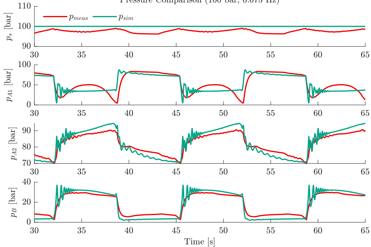
Pressure Comparison (100 bar, 0.075 Hz)
