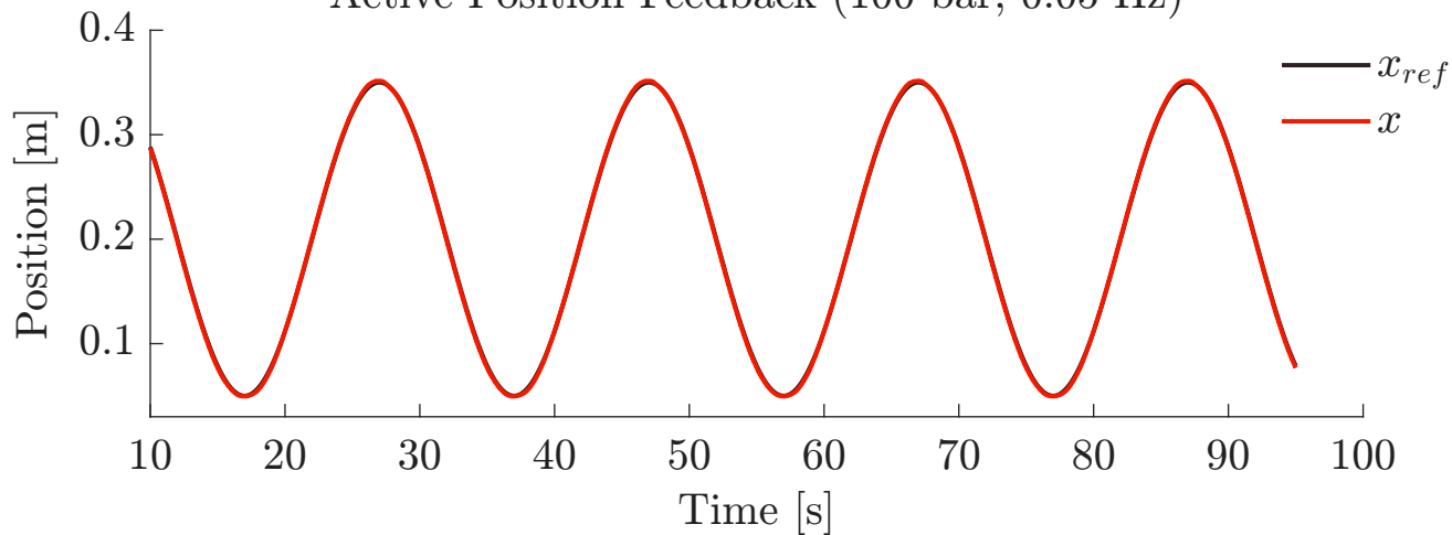
Active Position Feedback (100 bar, 0.05 Hz)
