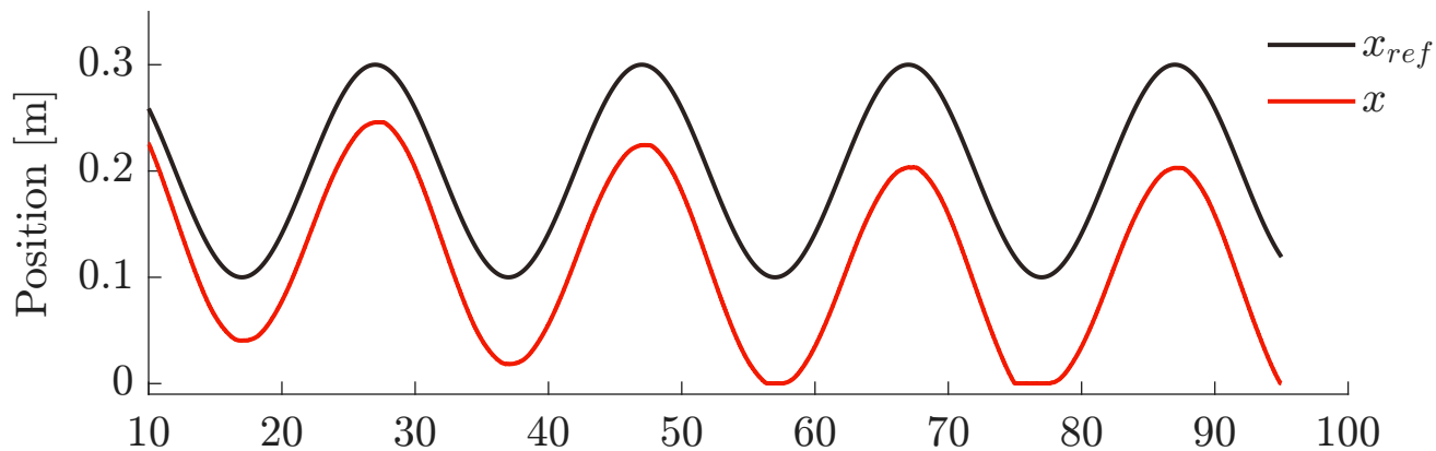
No Position Feedback (100 bar, 0.05 Hz)
