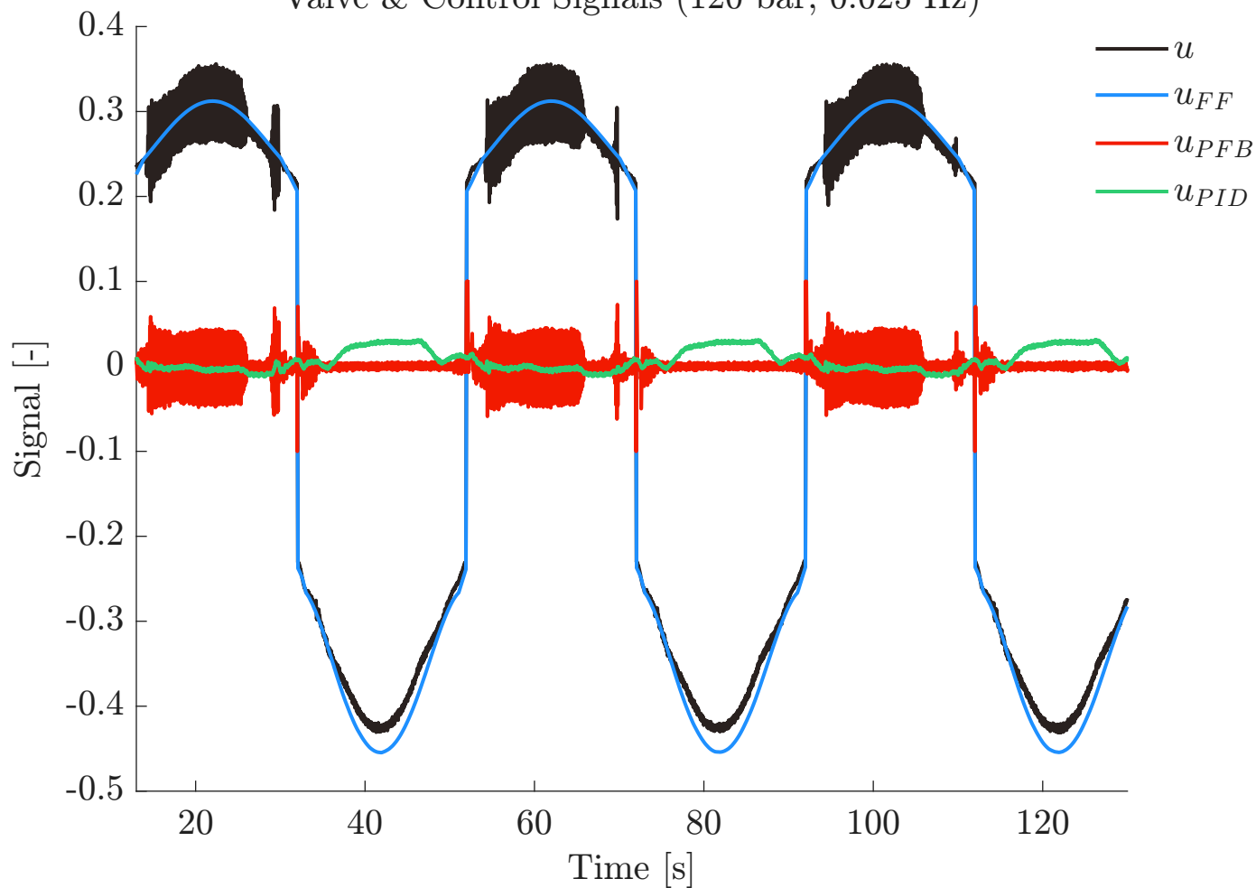
Valve & Control Signals (120 bar, 0.025 Hz)
