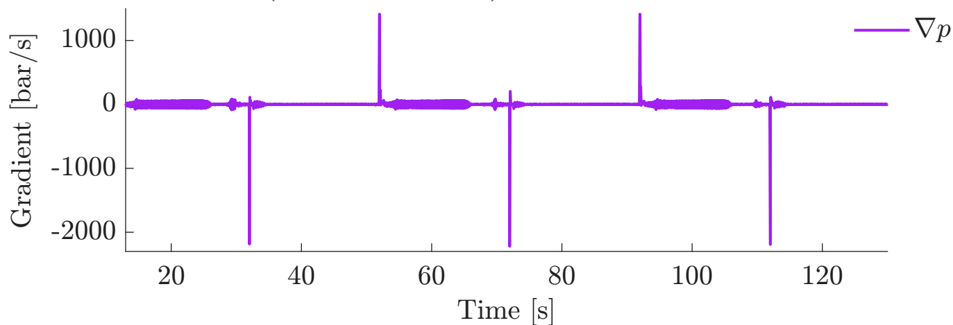
(120 bar, 0.025 Hz) - Pressure Gradient
