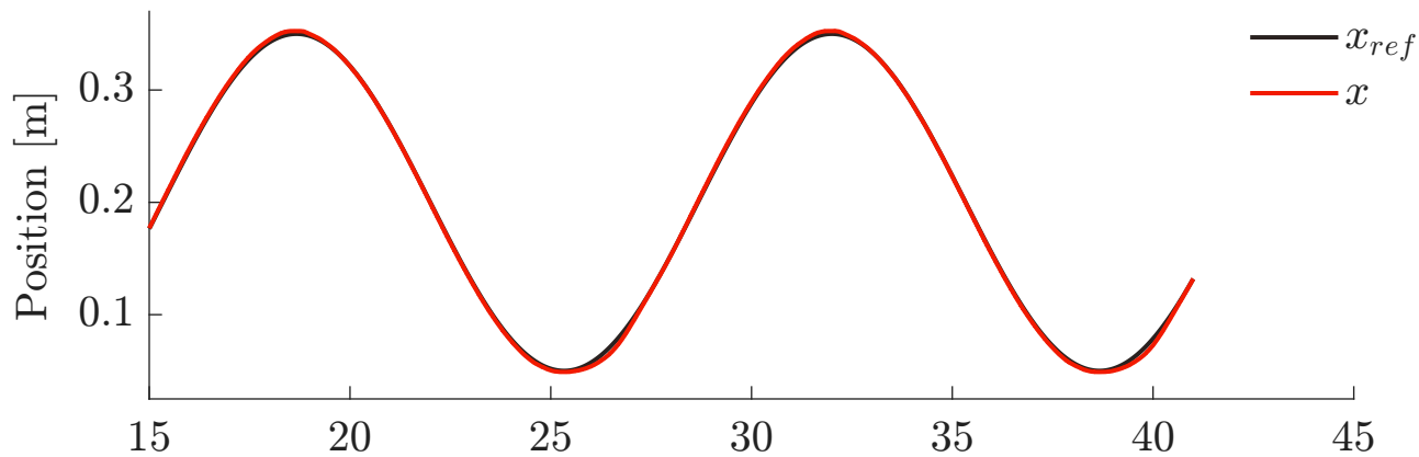
Active Kv FF (100 bar, 0.075 Hz)
