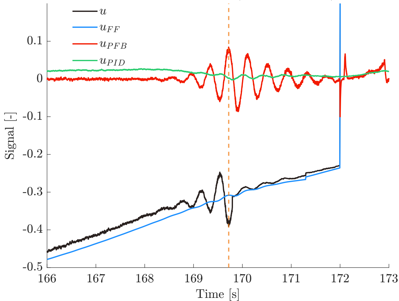
Valve & Control Signals (100 bar, 0.05 Hz)
