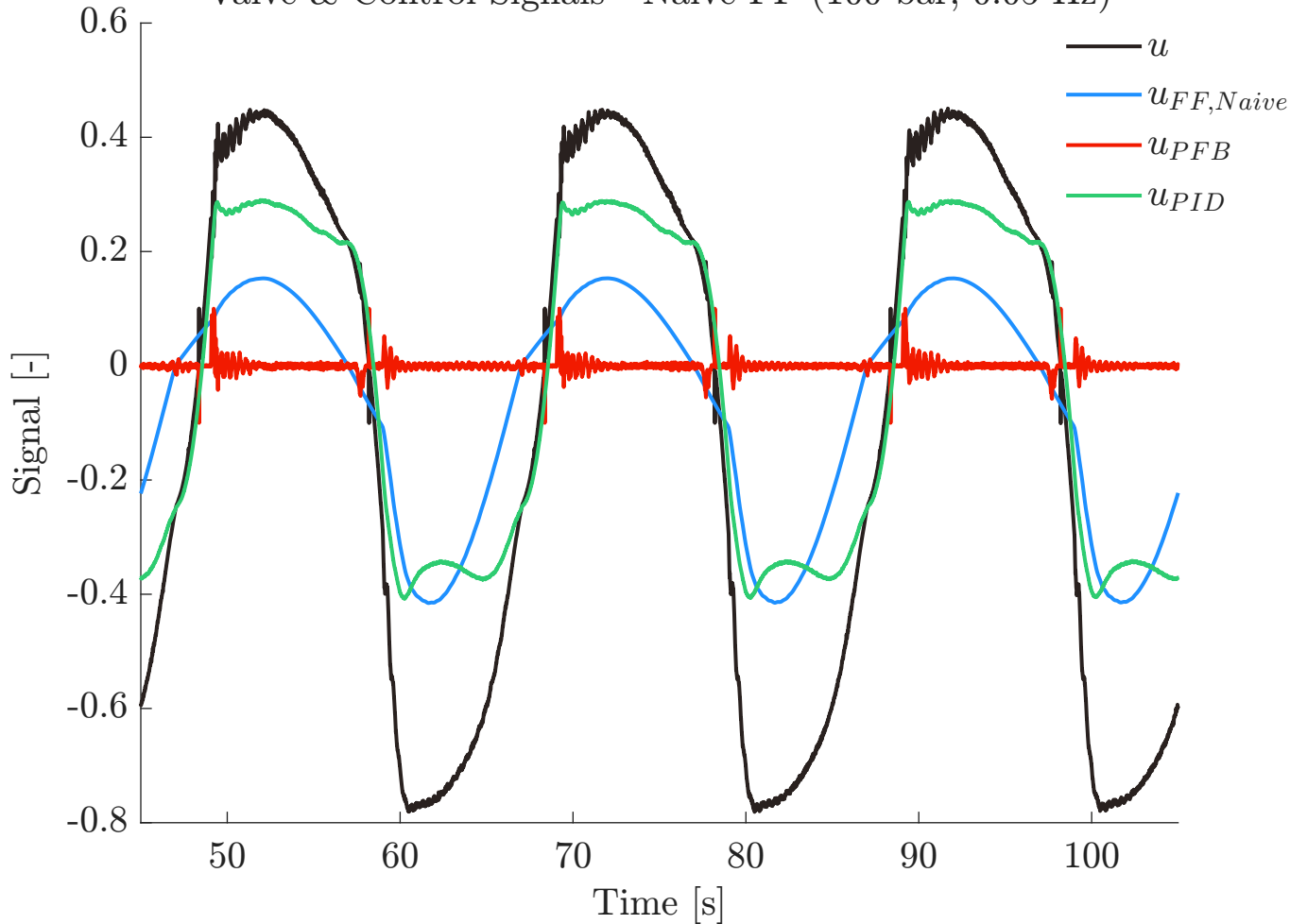
Valve & Control Signals - Naive FF (100 bar, 0.05 Hz)
