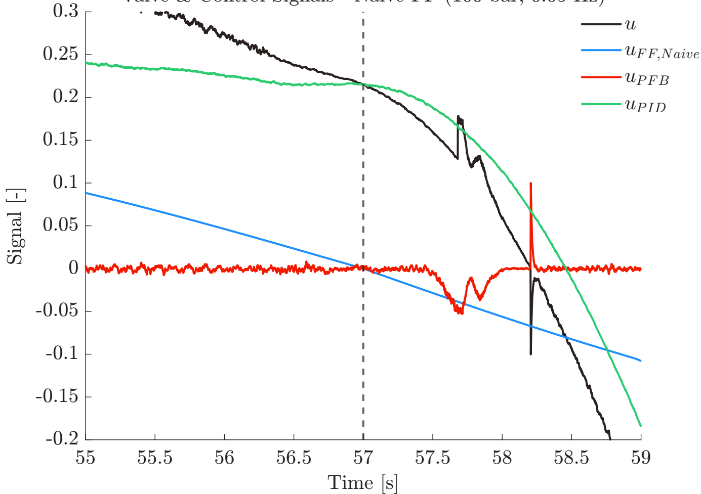
Valve & Control Signals - Naive FF (100 bar, 0.05 Hz)
