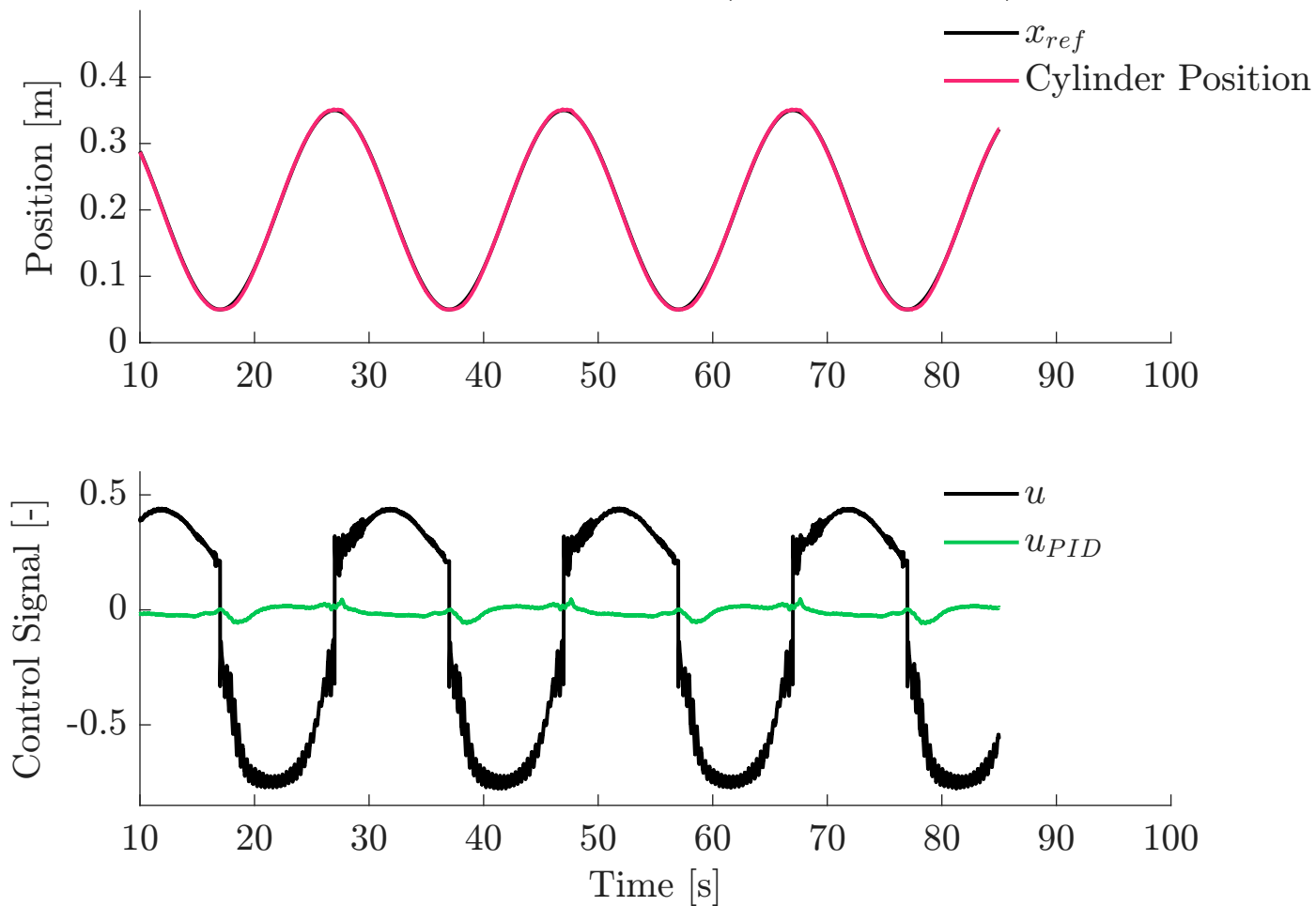
Active Position Feedback (100 bar, 0.05 Hz)
