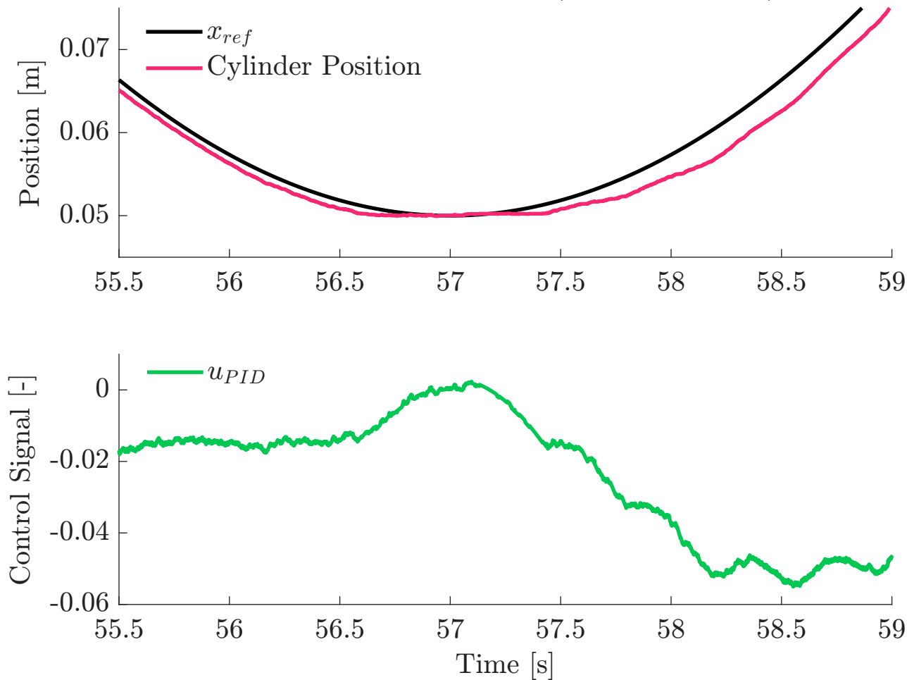
Active Position Feedback (100 bar, 0.05 Hz)
