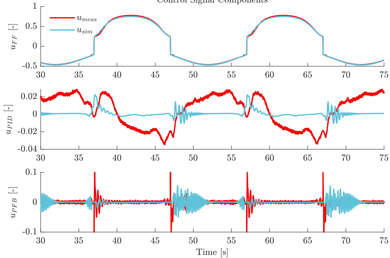
Control Signal Components
