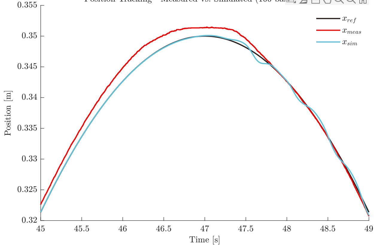
Position Tracking - Measured vs. Simulated (100 bar)
