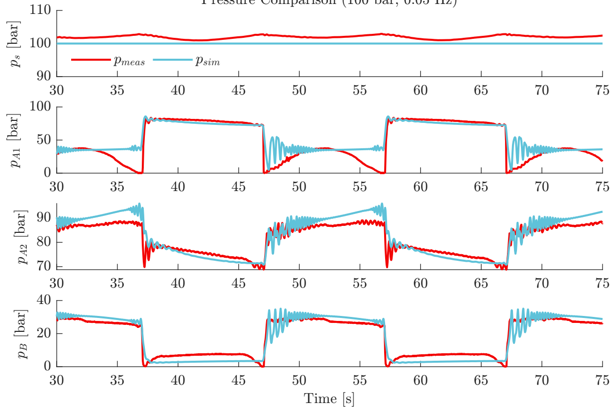
Pressure Comparison (100 bar, 0.05 Hz)
