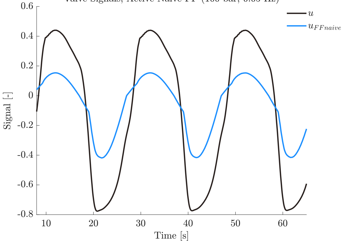
Valve Signals, Active Naive FF (100 bar, 0.05 Hz)
