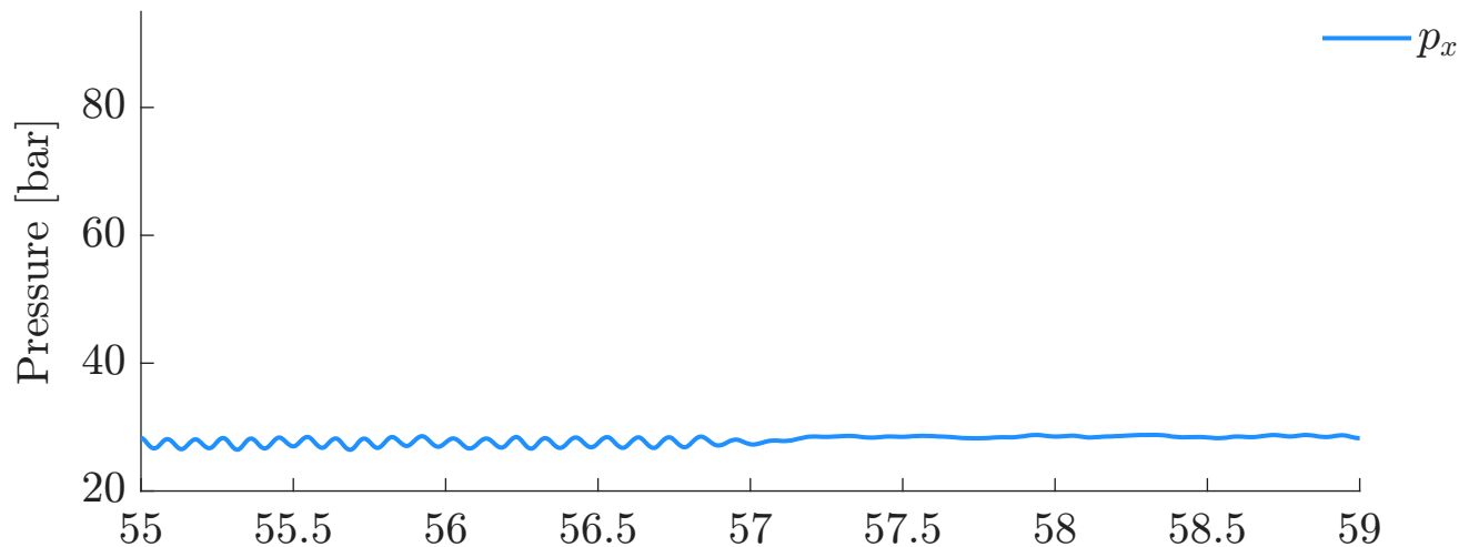
Pressure Feedback (100 bar, 0.05 Hz) - Selected Pressure
