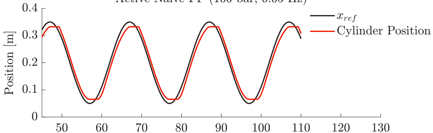
Active Naive FF (100 bar, 0.05 Hz)
