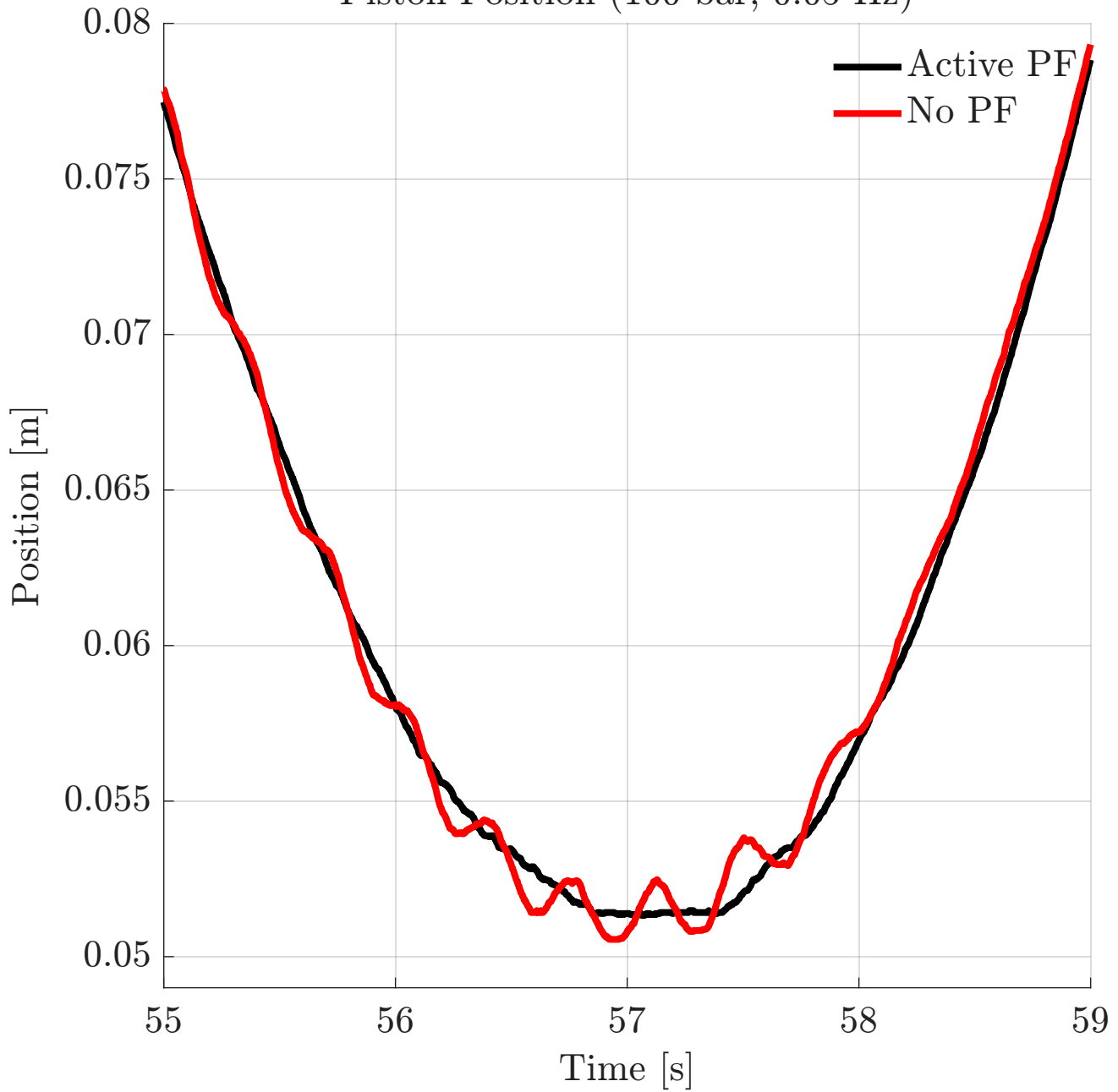
Piston Position (100 bar, 0.05 Hz)
