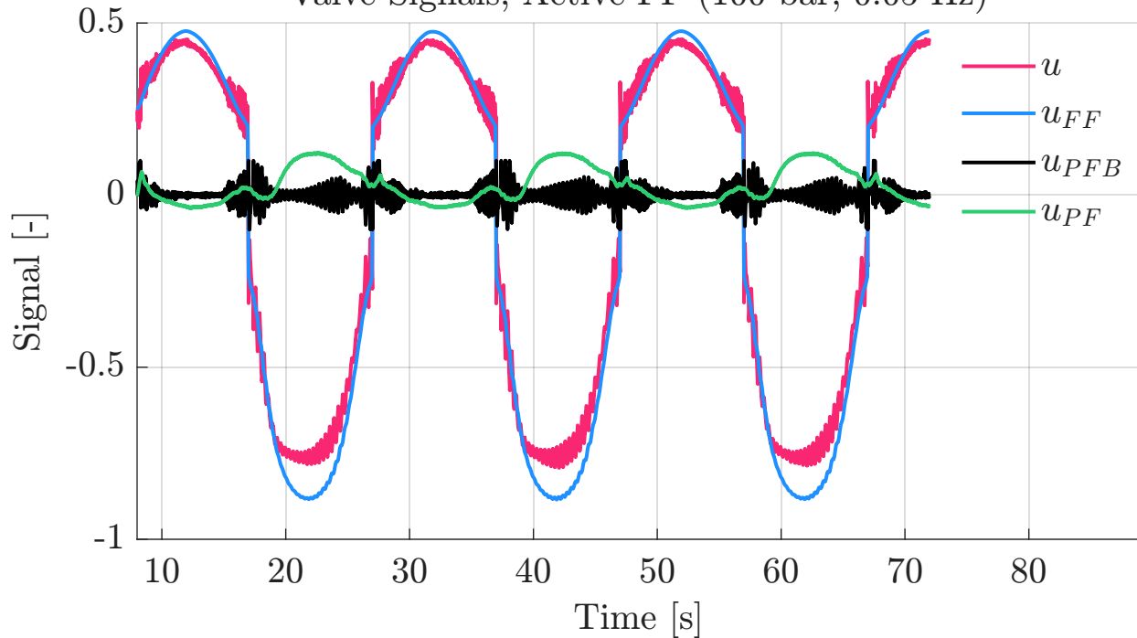
Valve Signals, Active FF (100 bar, 0.05 Hz)
