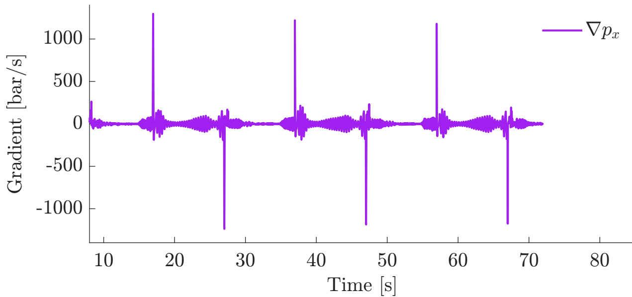
Pressure Feedback (100 bar, 0.05 Hz) - Pressure Gradient
