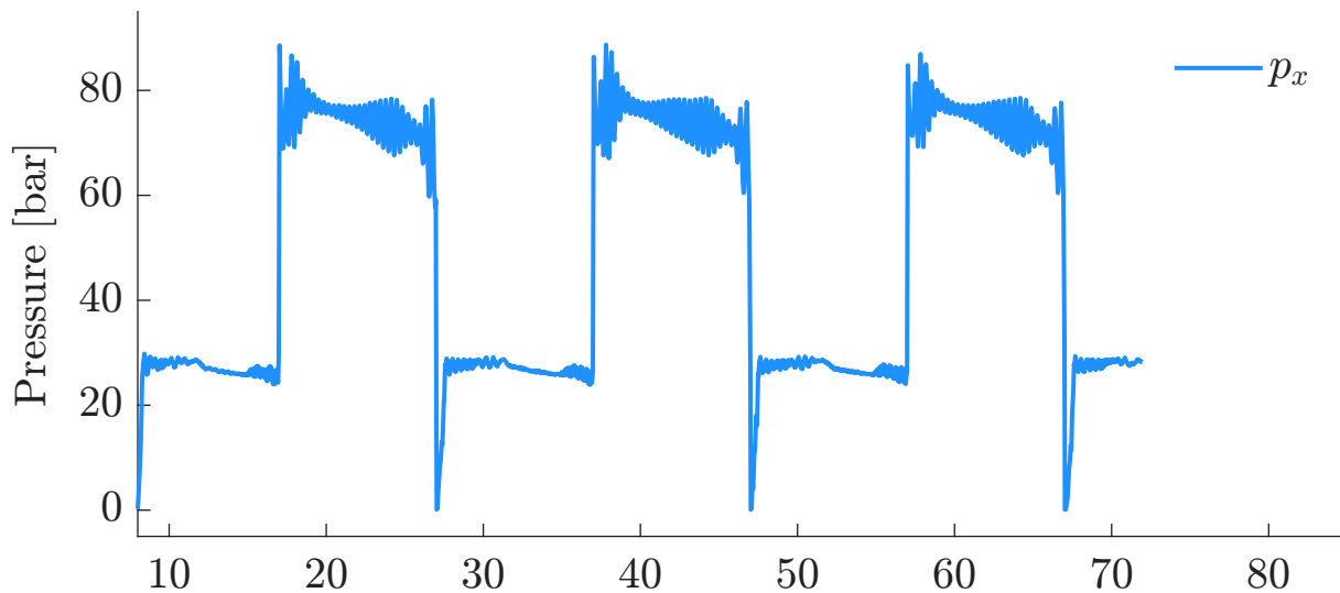
Pressure Feedback (100 bar, 0.05 Hz) - Selected Pressure
