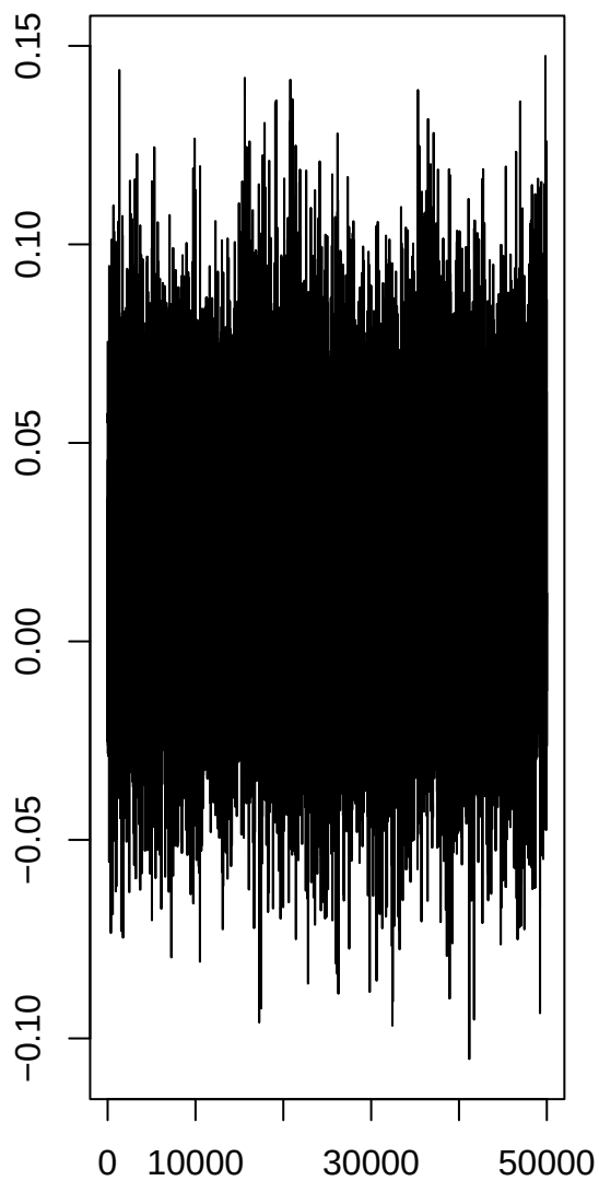
alpha
