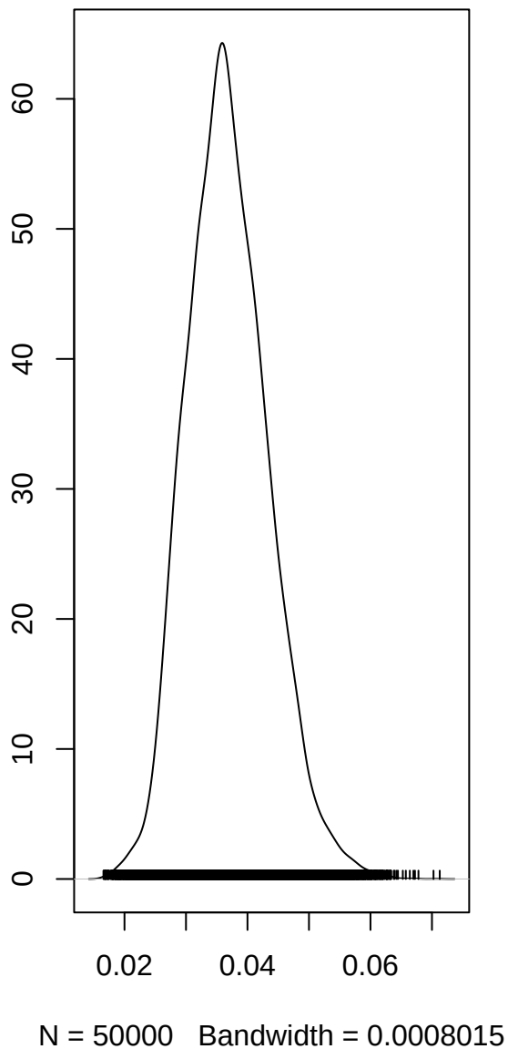
tau2.slo
