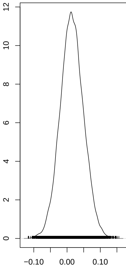
psych_rate
