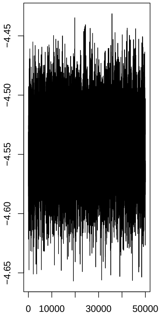
Intercept
