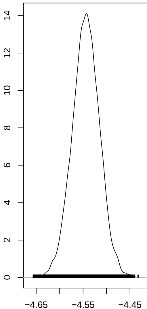
Intercept
