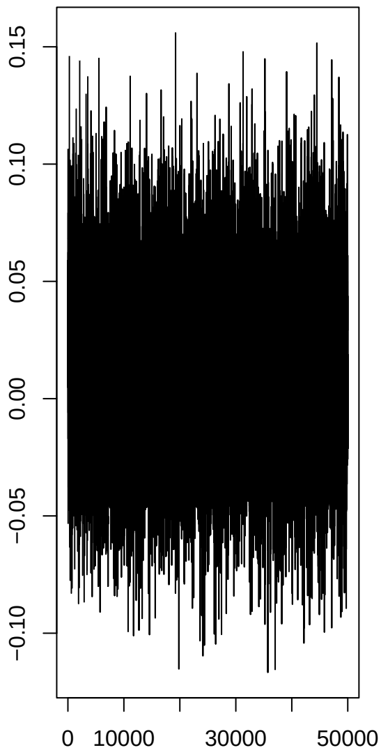
psych_rate
