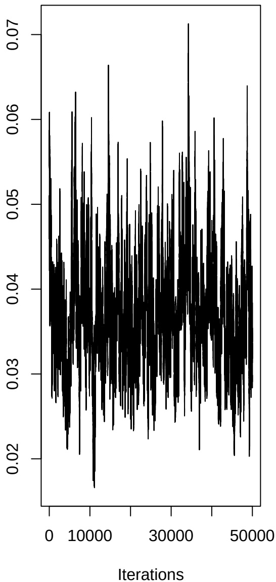
tau2.slo
