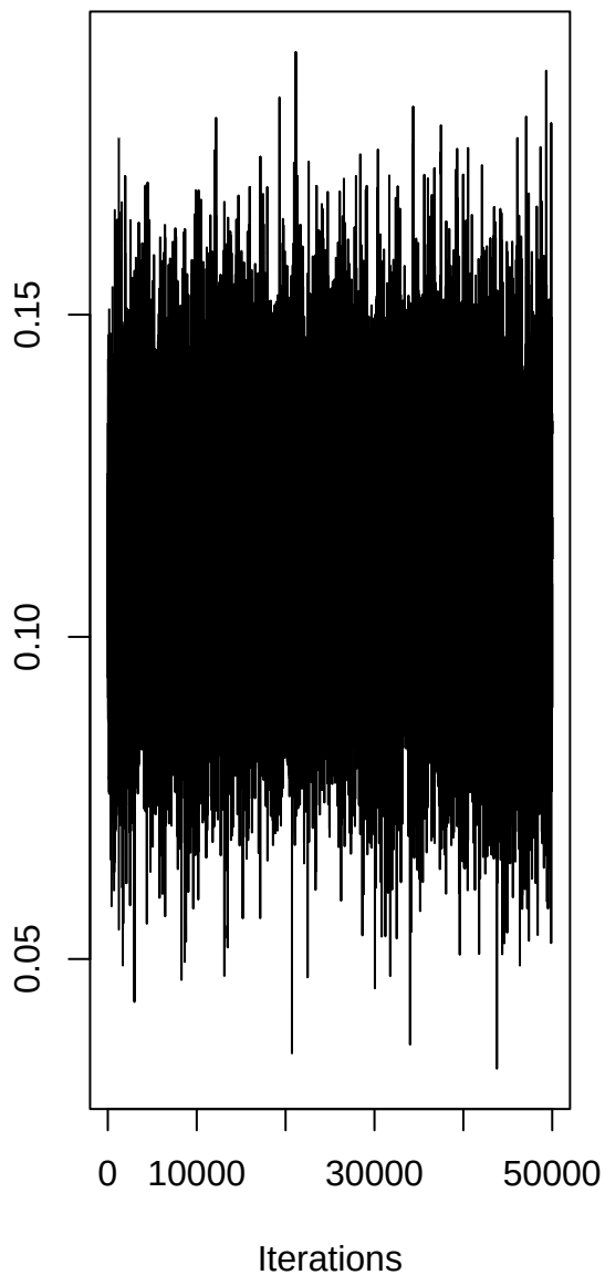
alpha
