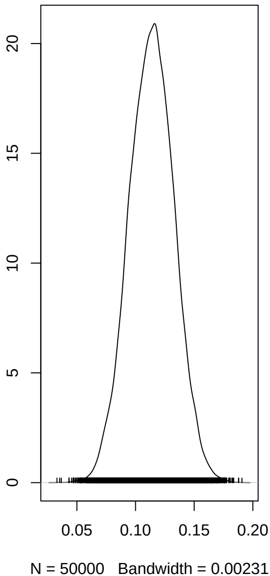
alpha
