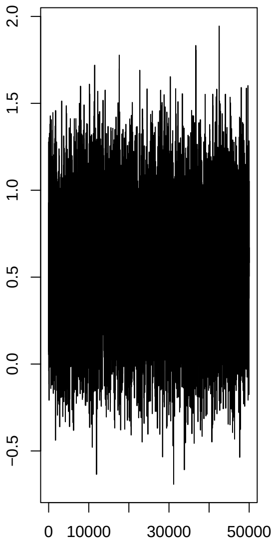
psych_rate
