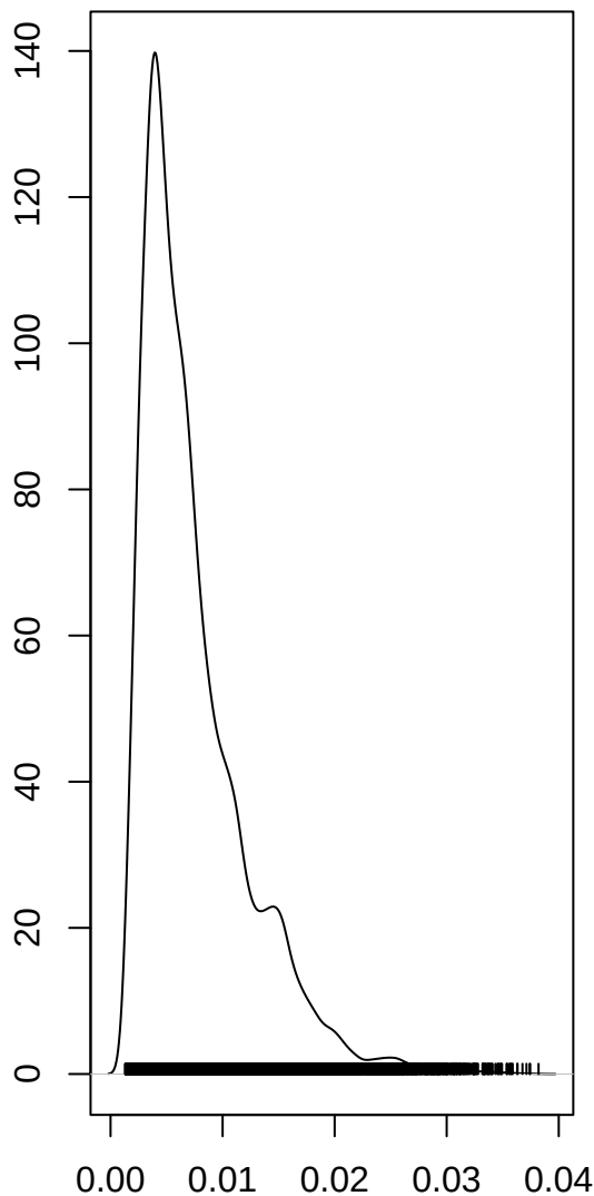
tau2.slo
