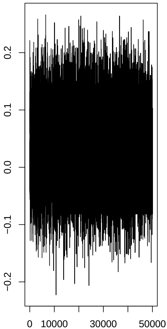
alpha
