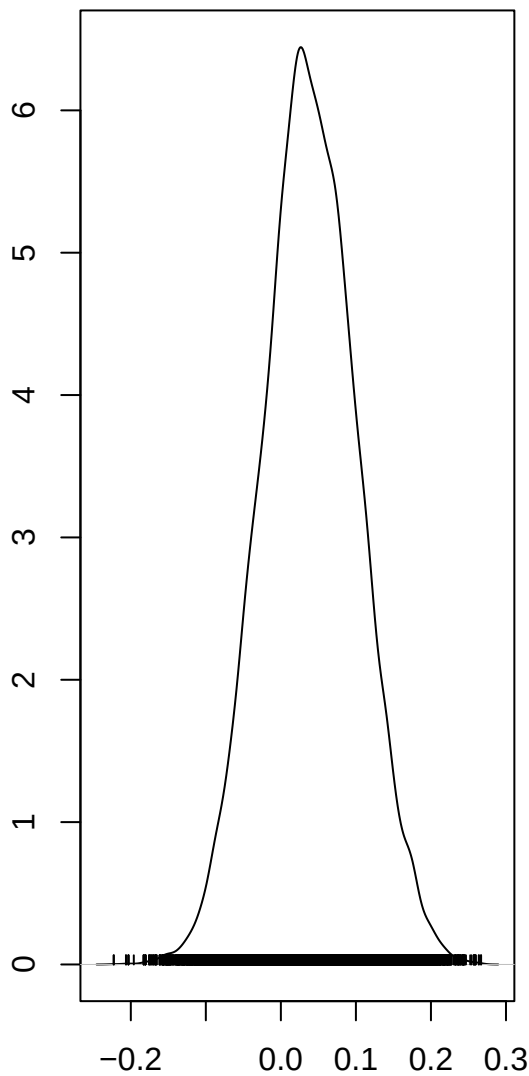
alpha
