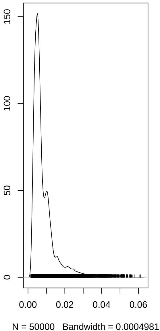
tau2.slo
