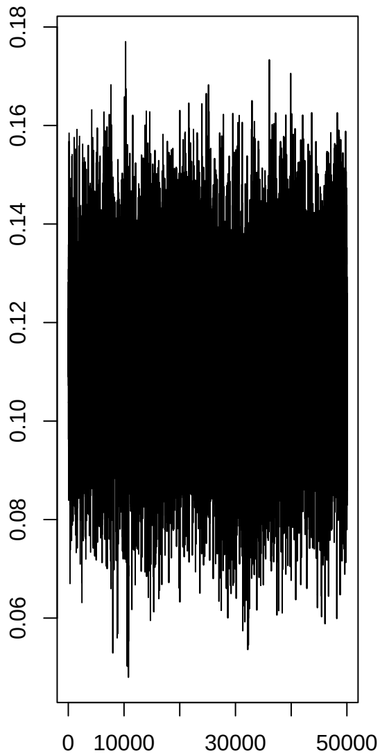
alpha
