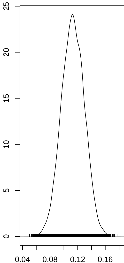
alpha
