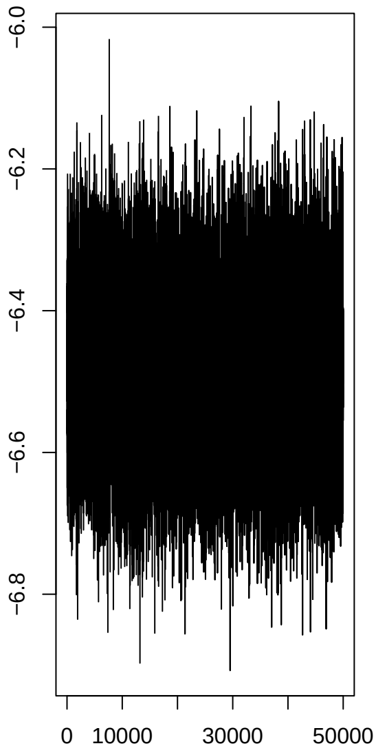
Intercept
