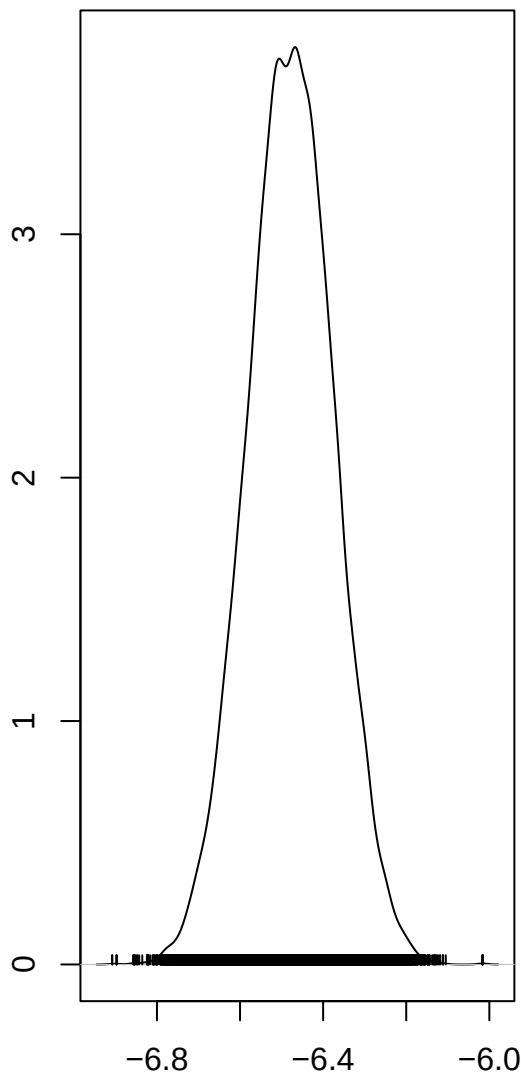
Intercept
