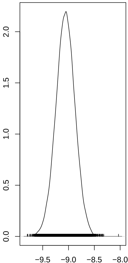
Intercept
