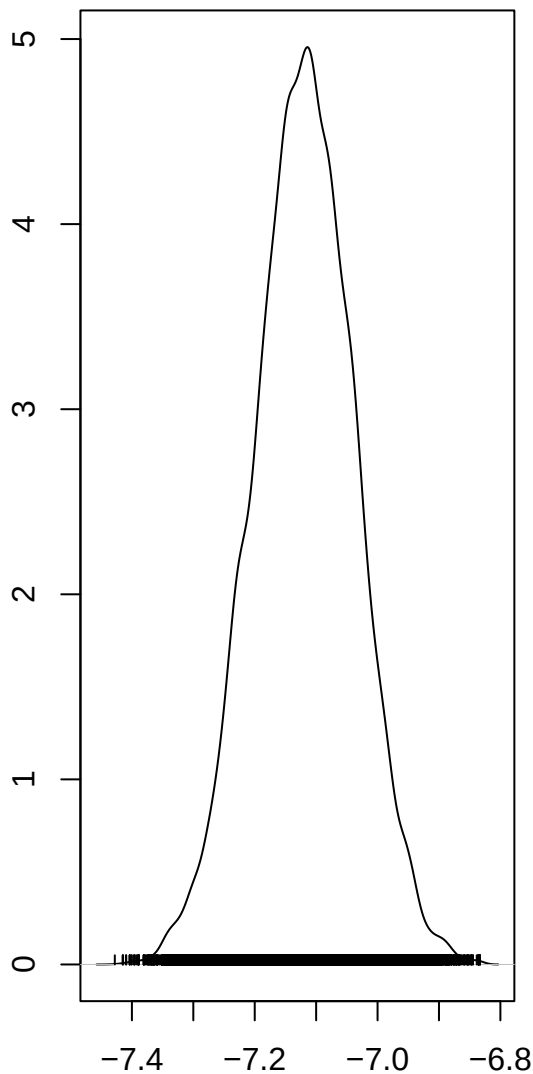
Intercept
