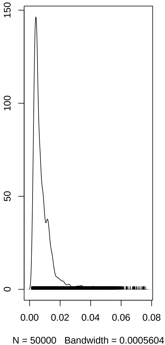
tau2.slo
