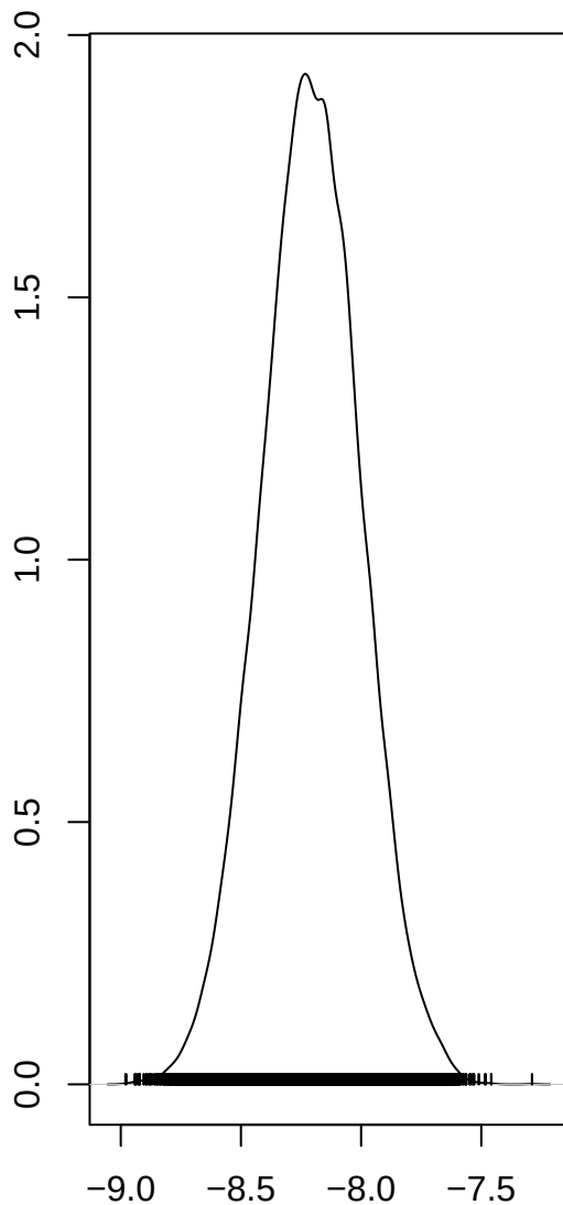
Intercept
