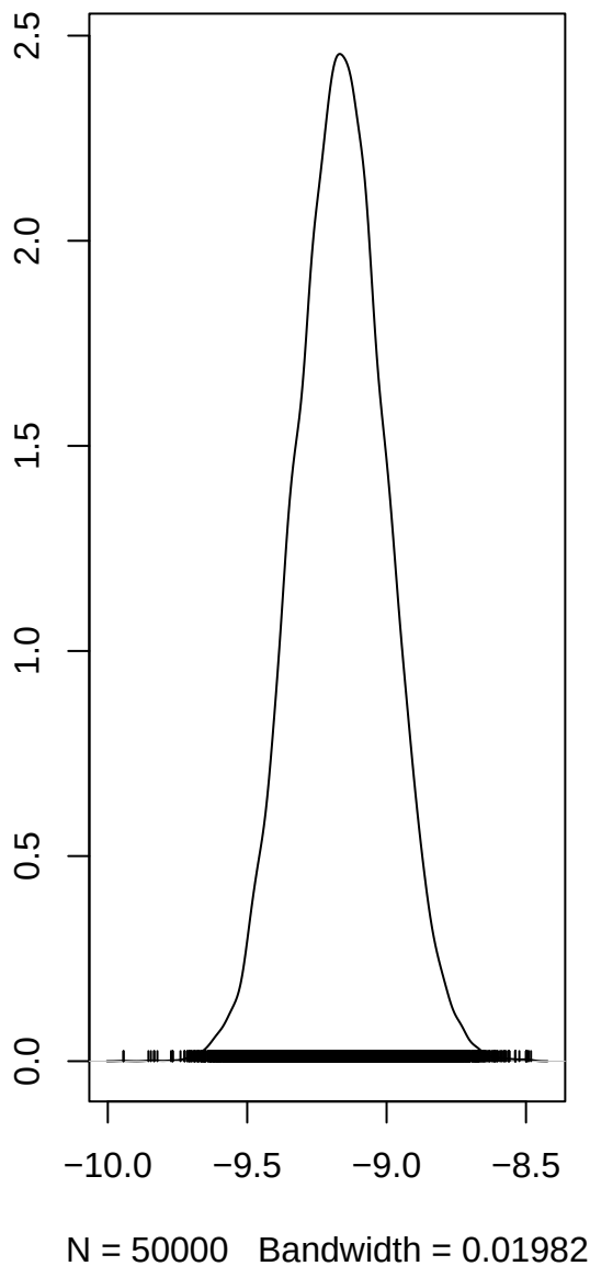
Intercept
