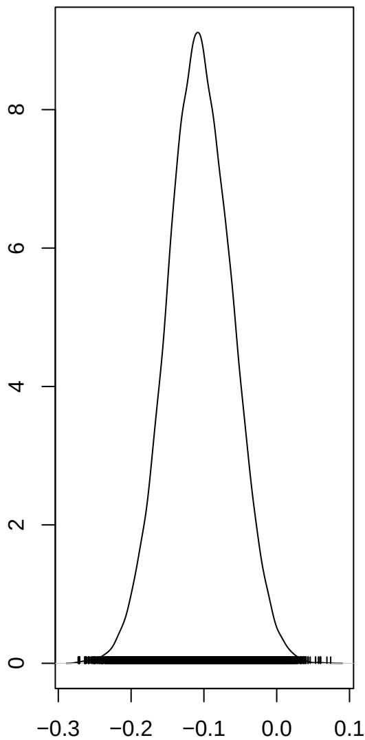
alpha
