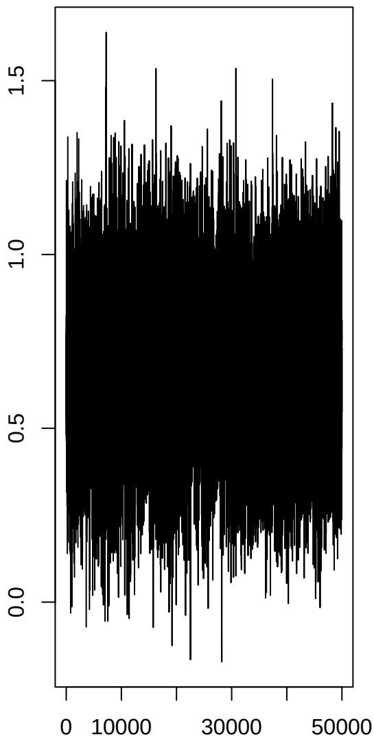
psych_rate
