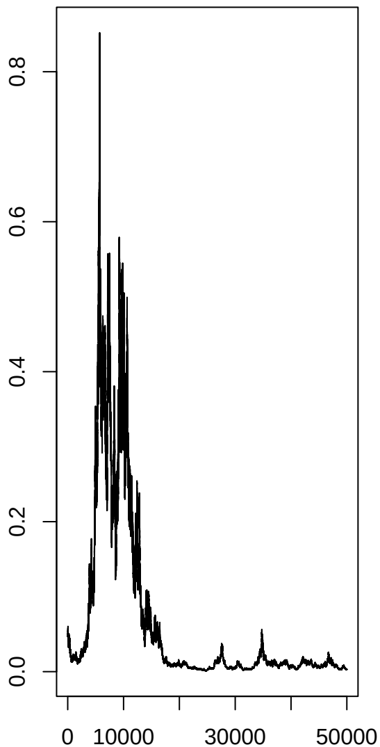
tau2.slo
