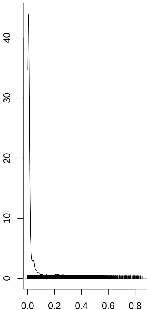
tau2.slo
