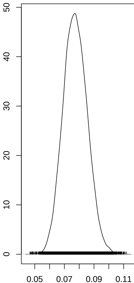
tau2.slo
