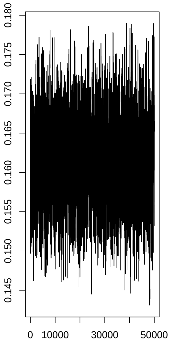
alpha
