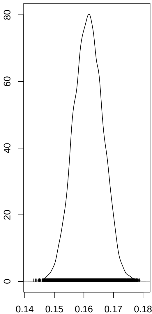
alpha
