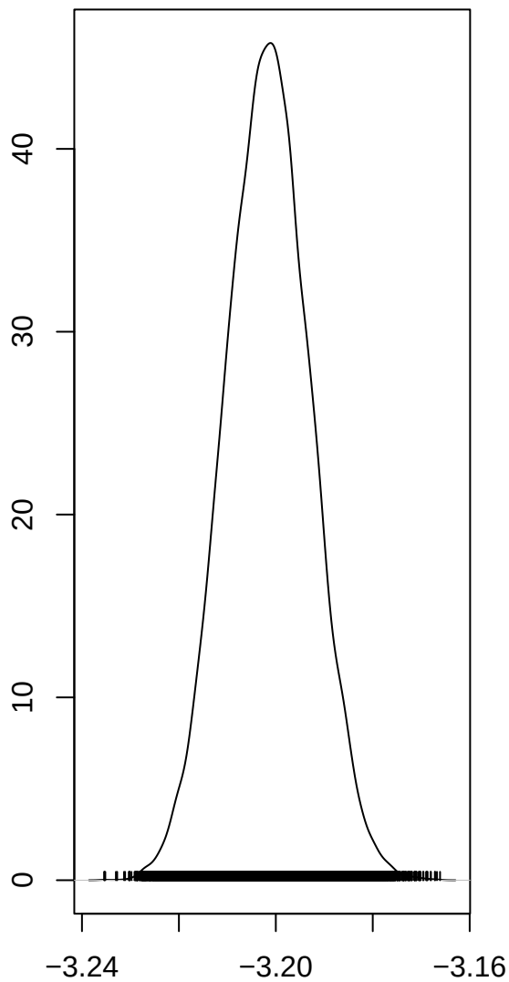
Intercept
