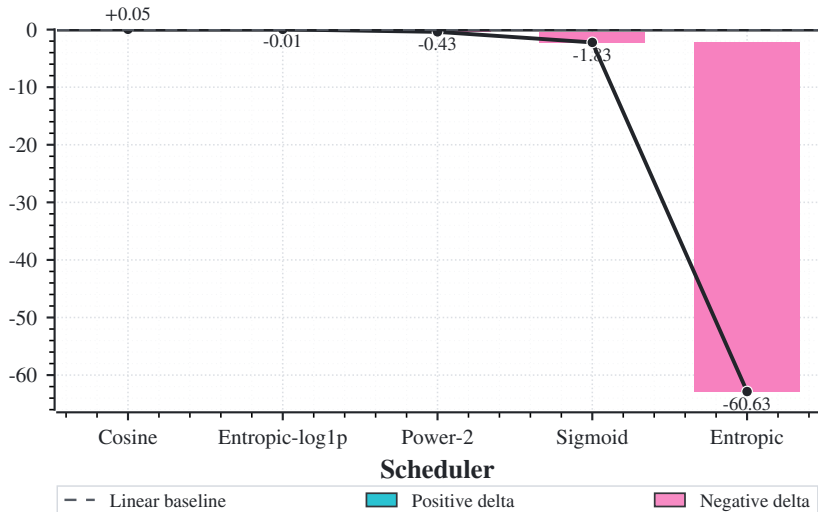
FID change vs linear at 25 NFE
