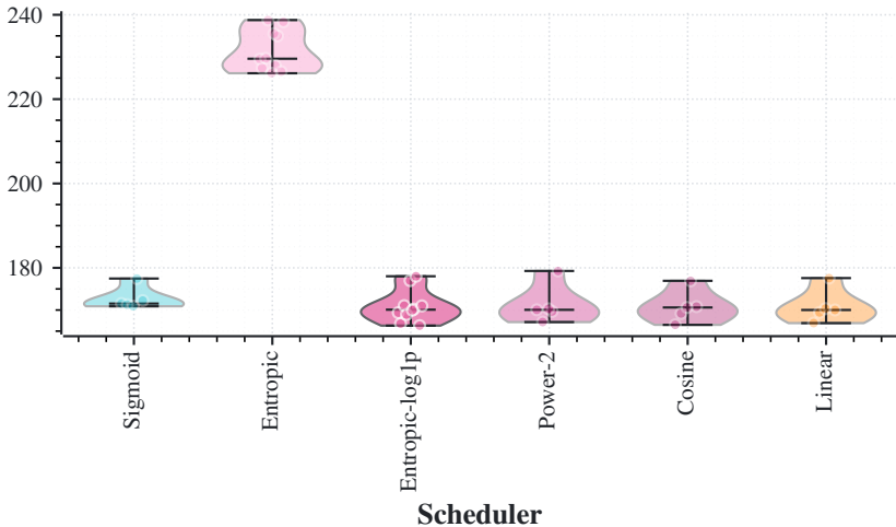
Inception FID
