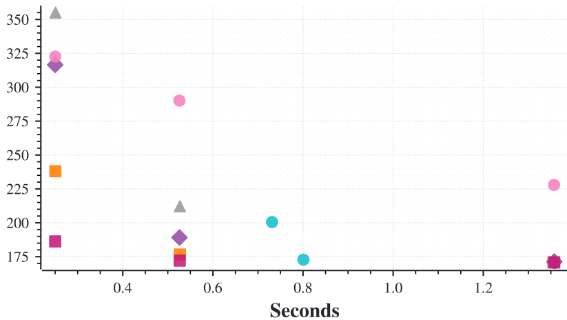
Inception FID
