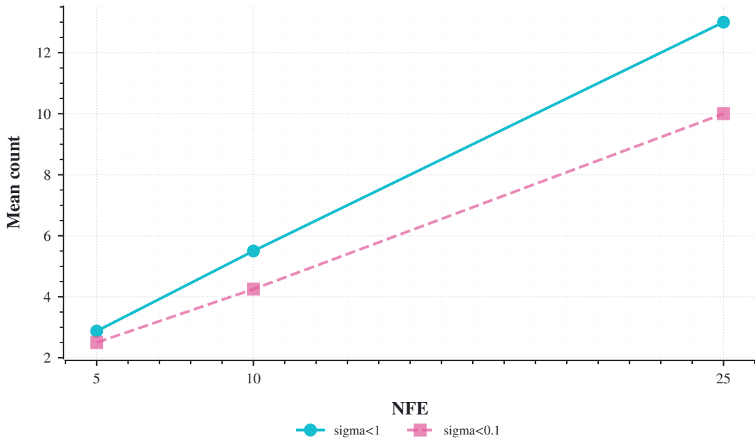
run40 EDM ode heun threshold allocation
