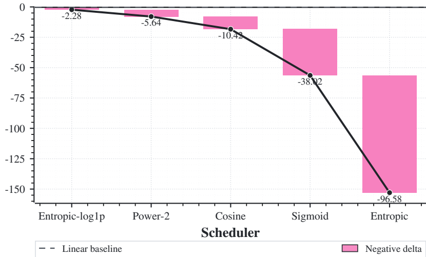
FID change vs linear at 25 NFE
