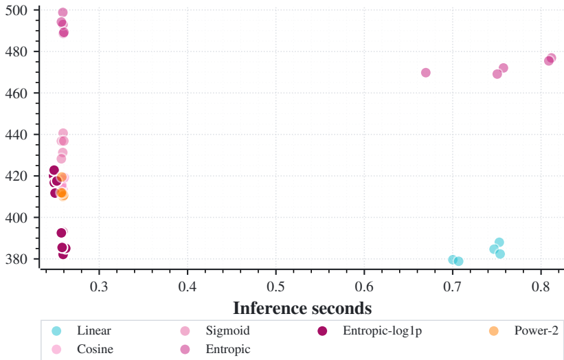
Inception FID
