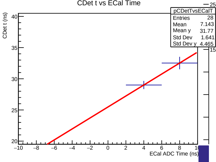
CDet Layer 2 t vs ECal Time
