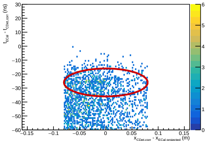
Pairless one-layer events, Layer 1 good pulses
