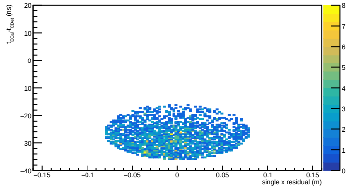
SBSCDet single_candidate.*
