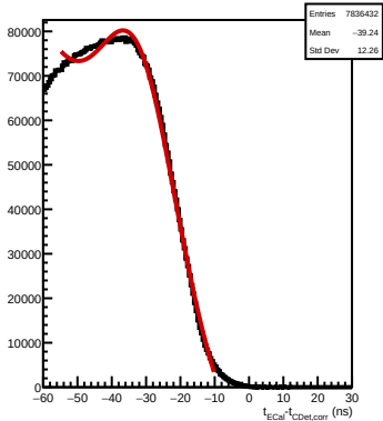
Old: ECal energy cut, events with an accepted CDet pair
