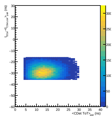
Old: trajectory-time selected pair mean, all CDet
