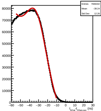
Native: ECal energy cut, events with an accepted CDet pair
