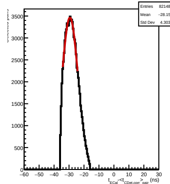
Native: trajectory-time selected pair mean, all CDet
