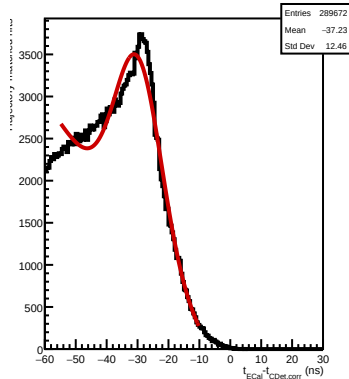
Native: projection-matched pulses, events with an accepted CDet pair
