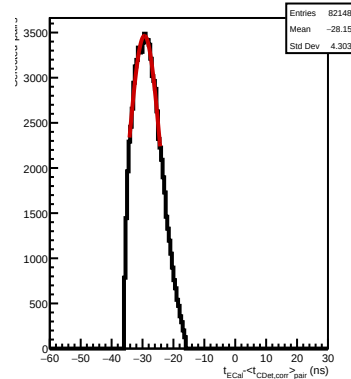
Old: trajectory-time selected pair mean, all CDet
