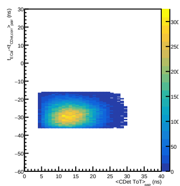
Native: trajectory-time selected pair mean, all CDet
