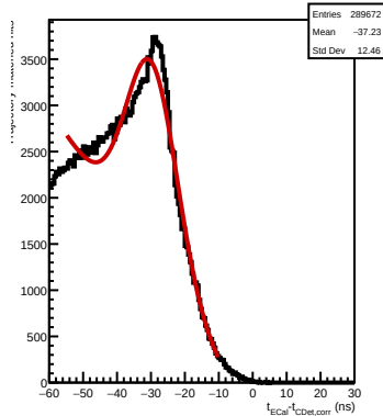
Old: projection-matched pulses, events with an accepted CDet pair
