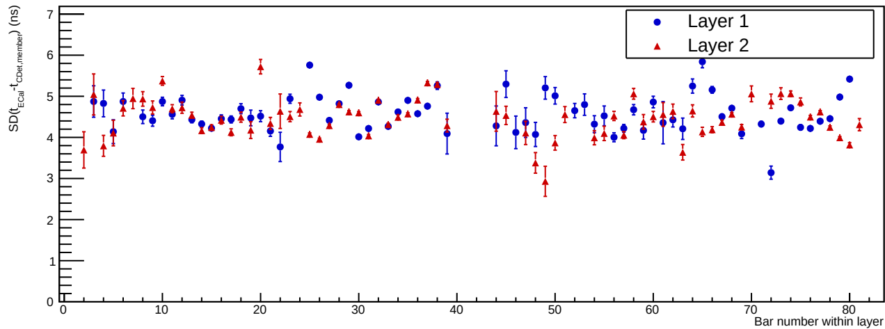
Run 6077: best-pair timing widths
