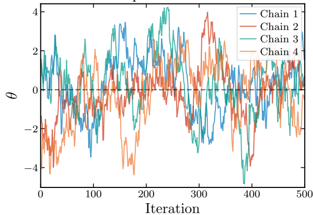
Multiple chains: \hat{R} \approx 1
