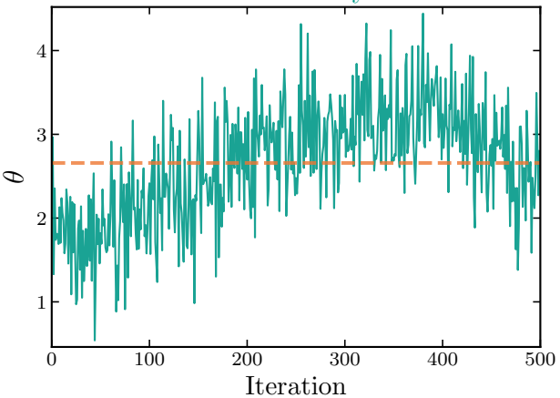
Good: stationary noise
